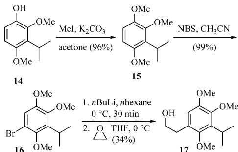
Scheme 1. Synthesis of the bromobenzene derivative 16 from phenol 14 .
