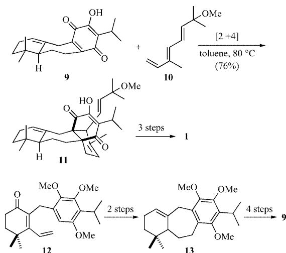
Figure 3. Key steps in the synthesis of salvadione ( 1 ) according to Majetich et al.
