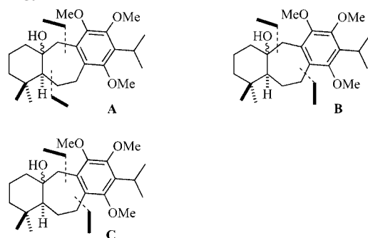
Figure 4. Possible disconnections in the central seven-membered ring.
