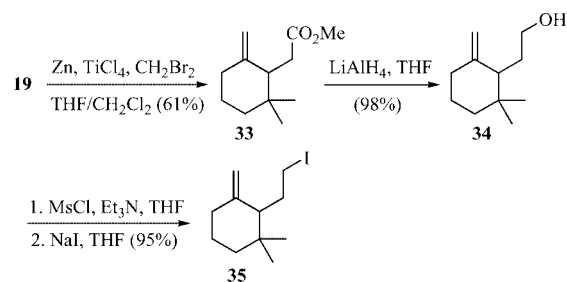
Scheme 5. Synthesis of the alkenyliodide 35 .
