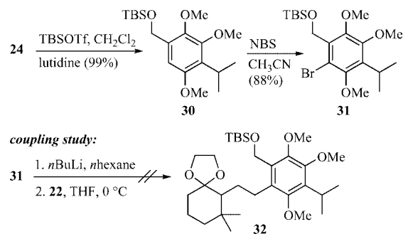
Scheme 4. Synthesis of the aryl bromide 31 and attempts to alkylate it with the iodide 22 .
