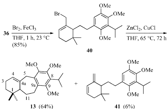
Scheme 7. Intramolecular Friedel–Crafts alkylation of allyl bromide 40 .
