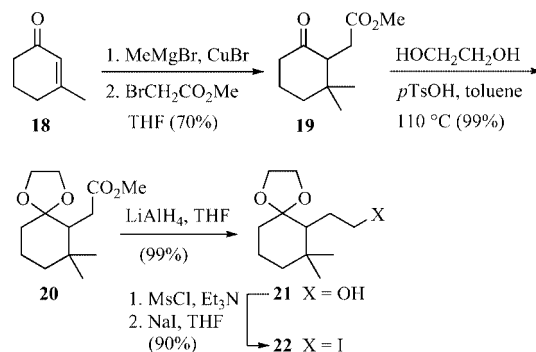
Scheme 2. Synthesis of the iodoalkane 22 from enone 18 .
