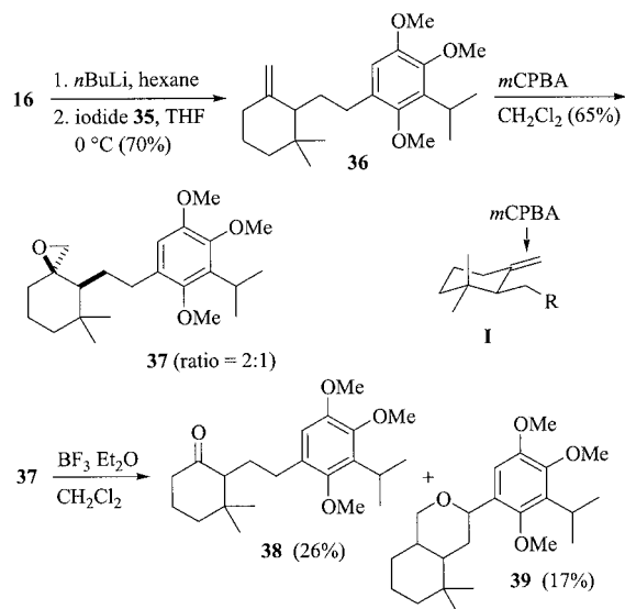
Scheme 6. Alkylation of the metalated benzene 16 with iodide 35 , and attempts to cyclize the derived epoxide 37 .
