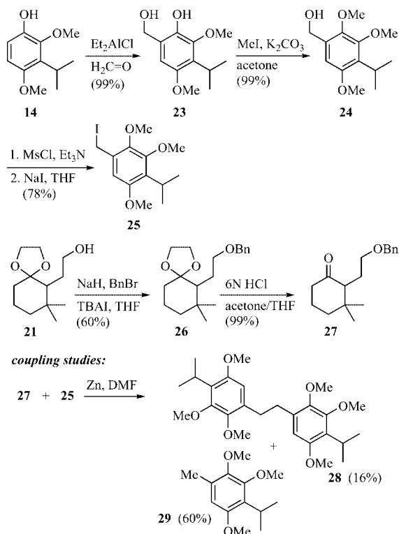
Scheme 3. Synthesis of the benzyl iodide 25 and its attempted coupling with cyclohexanone 27 .
