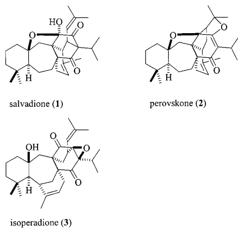
Figure 1. Structures of salvadione ( 1 ) and related compounds.
