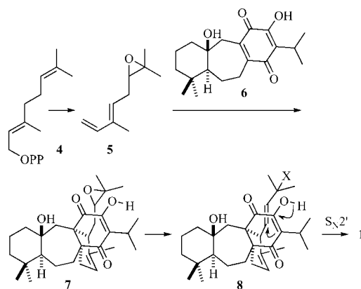
Figure 2. Proposed biosynthesis for salvadione ( 1 ) by an intermolecular Diels–Alder reaction.
